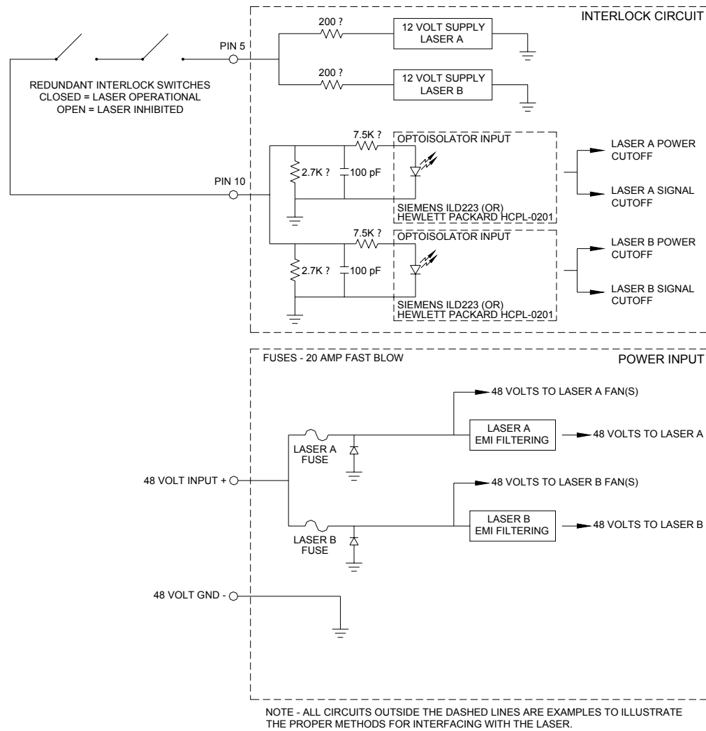
Figure 17b – Laser interconnect schematic Part B
