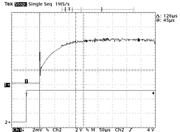
Figure 18 – Oscilloscope trace of typical rise time for a laser
