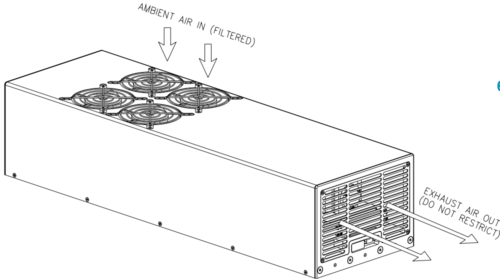
Figure 21 – Detail of air flow through the laser
