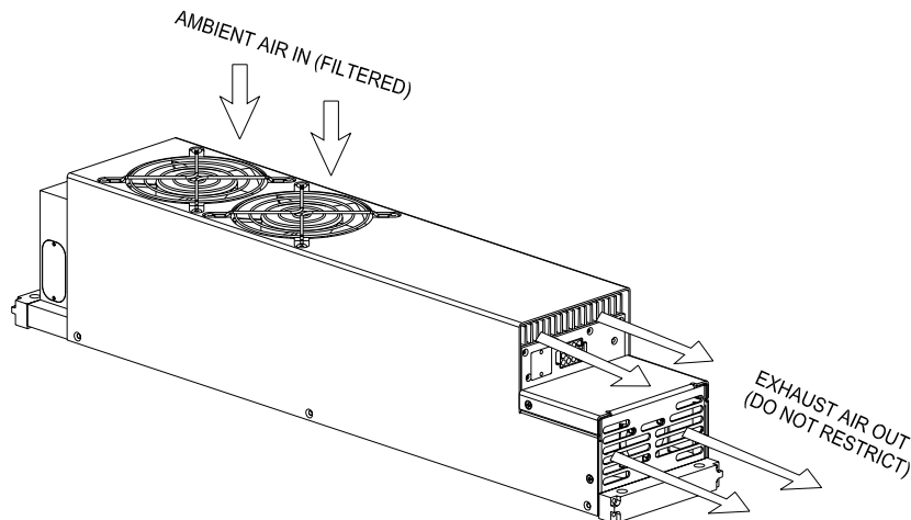
Figure 12 – Detail of air flow through the laser
