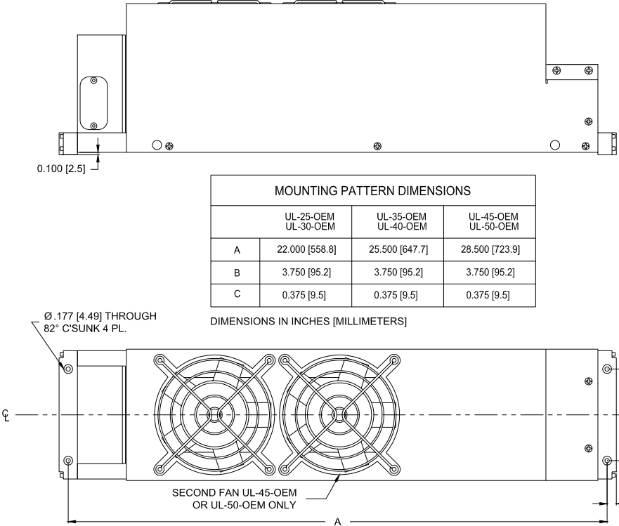
Figure 3 - Detail of mounting block dimensions
