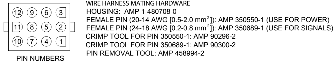
Figure 7 – Laser connector pin diagram
