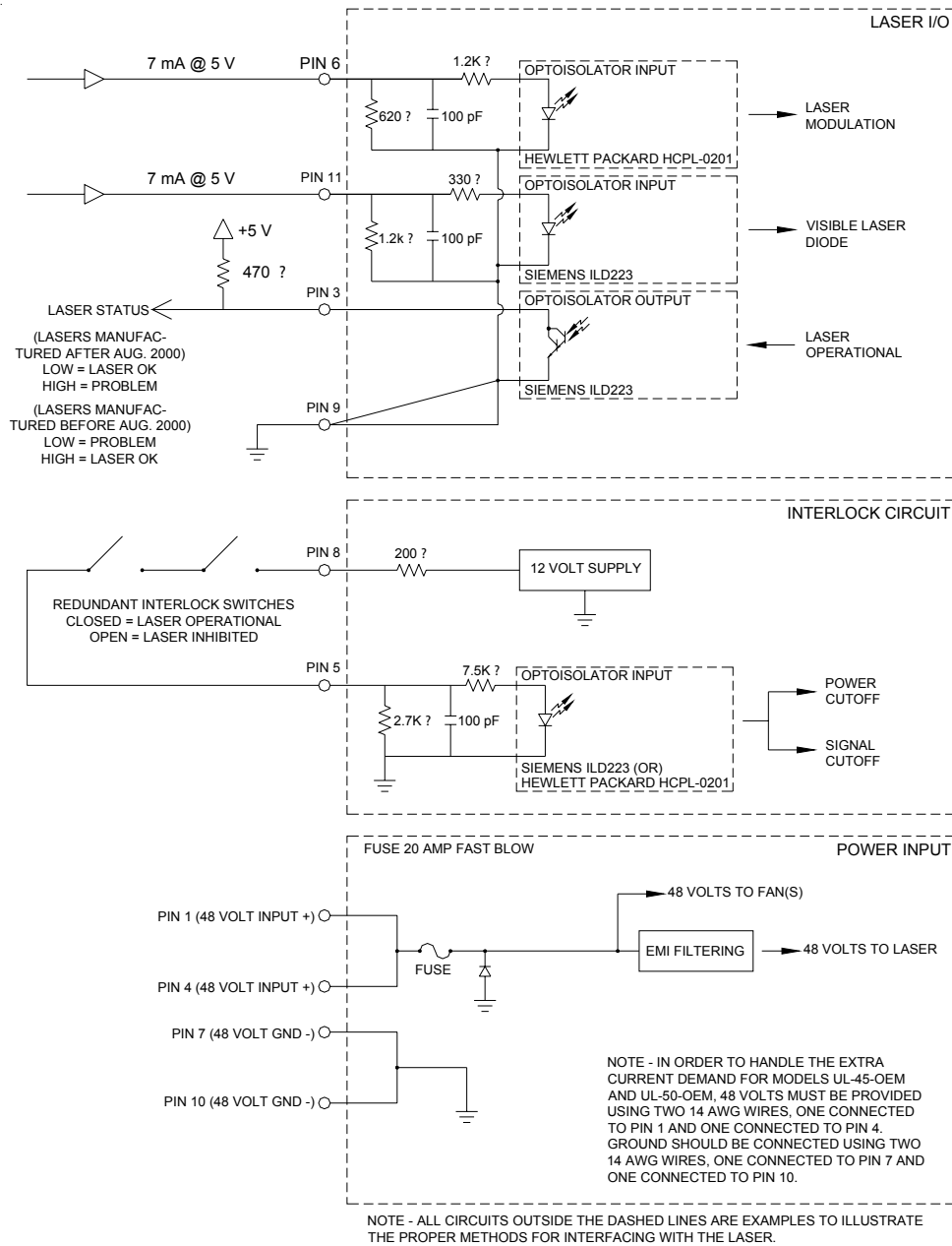
Figure 8 - Laser interconnect schematic
