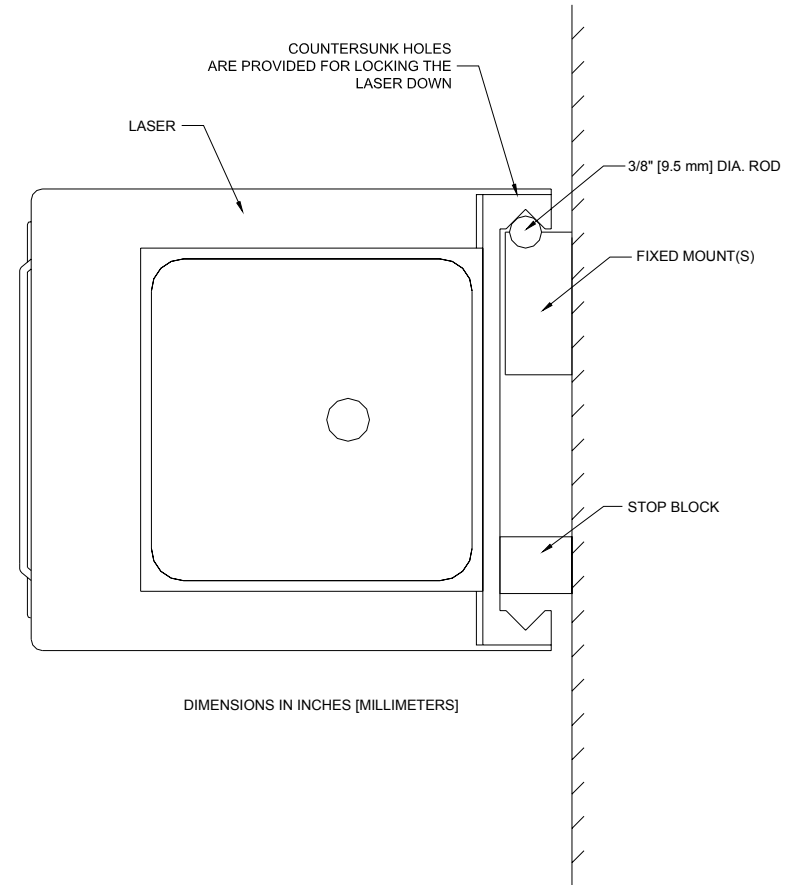
Figure 6 - Example of laser mounting using dovetail
