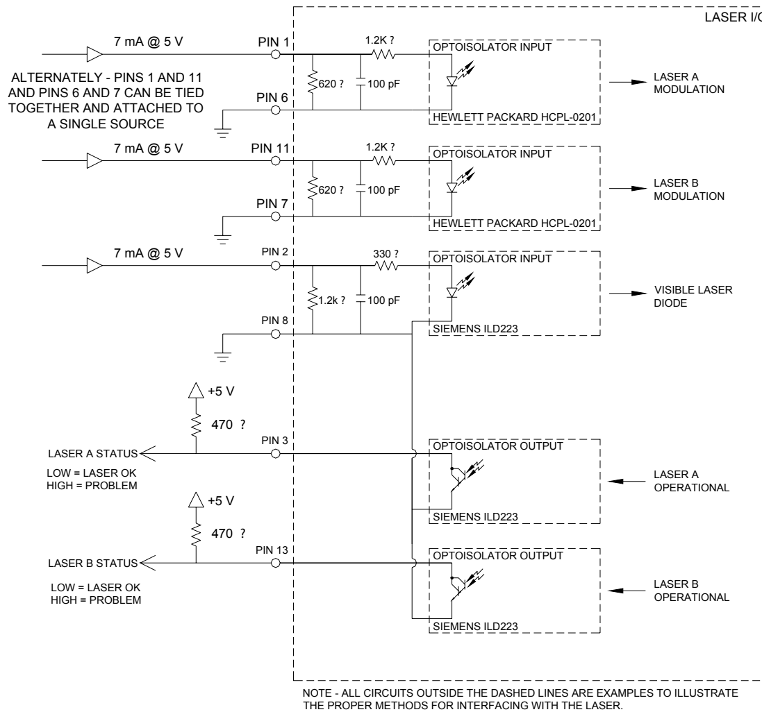
Figure 17a – Laser interconnect schematic Part A
