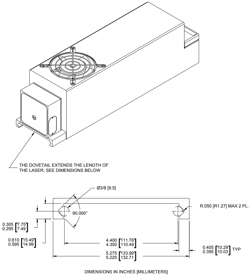
Figure 5 - Dovetail detail
