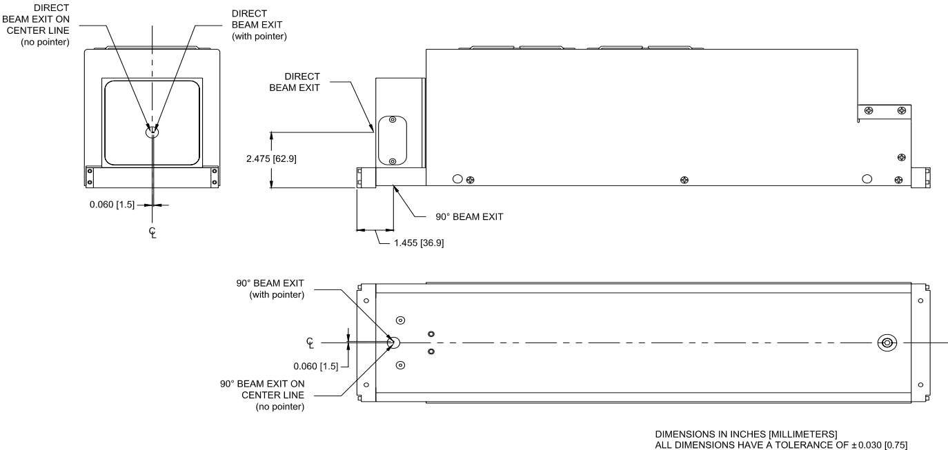
Figure 13 – Detail of Beam Output with and without pointer
