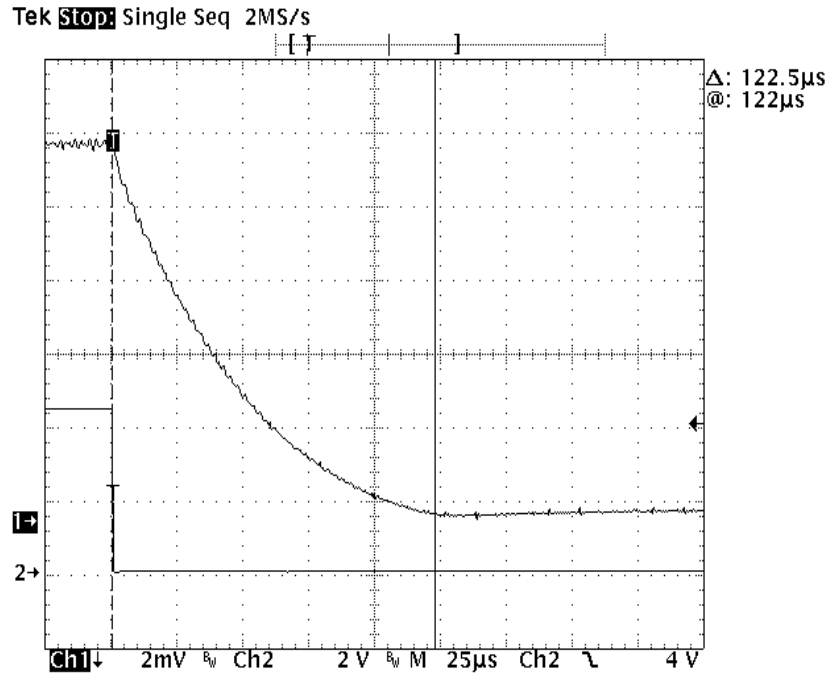
Figure 19 – Oscilloscope trace of typical fall time for a laser
