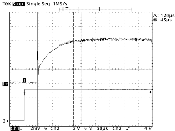
Figure 9 – Oscilloscope trace of typical rise time for a laser
