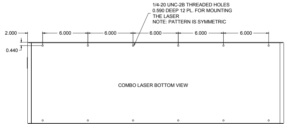
Figure 15 - Detail of mounting holes
