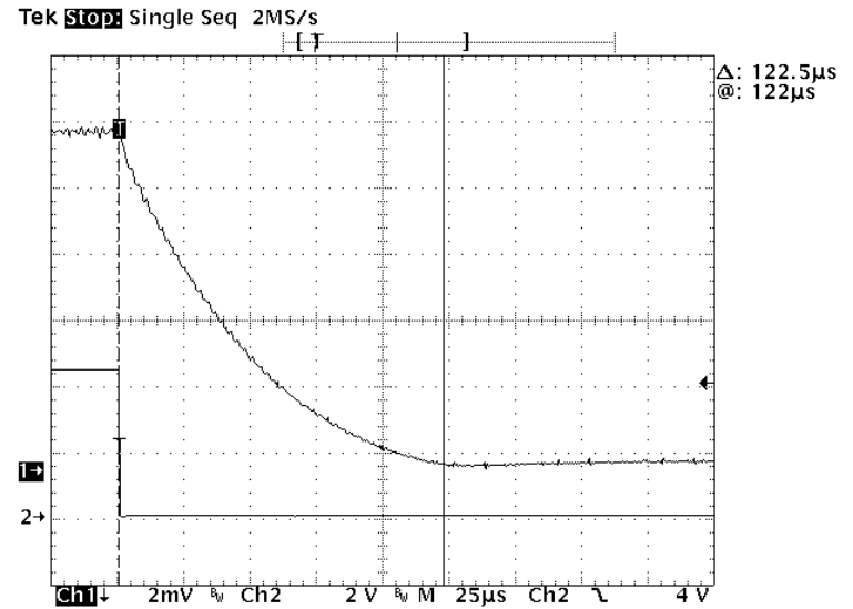
Figure 10 – Oscilloscope trace of typical fall time for a laser
