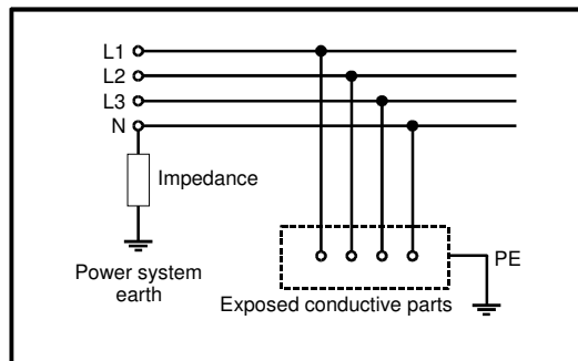
Example of IT power system
