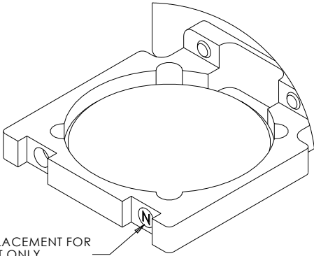
DETAIL N SCALE 3 : 1
